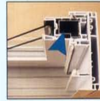
Metal reinforced sash provides structural strength.
