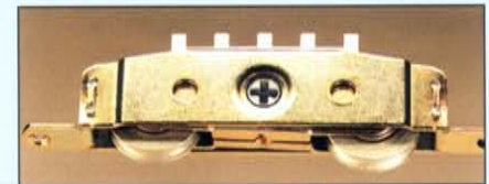
Our patio door glides on four heavy-duty brass rollers which provide long-lasting, trouble-free operation. The rollers are easy to adjust from the outside.
